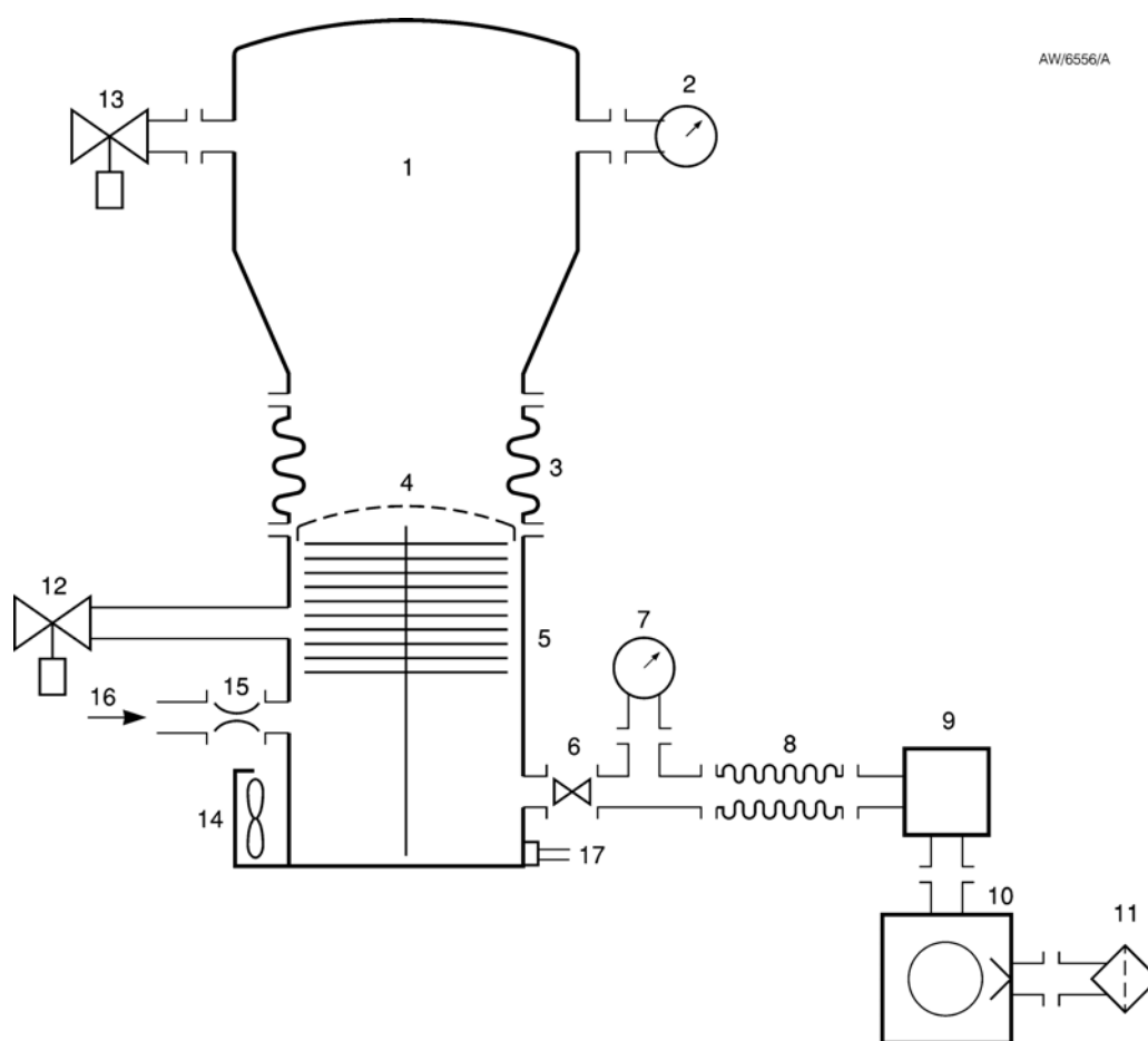
Figure 9 - Typical pumping system with a nEXT pump
