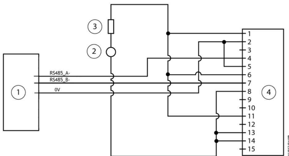
Figure 13 - Logic interface connections - RS485 serial mode
